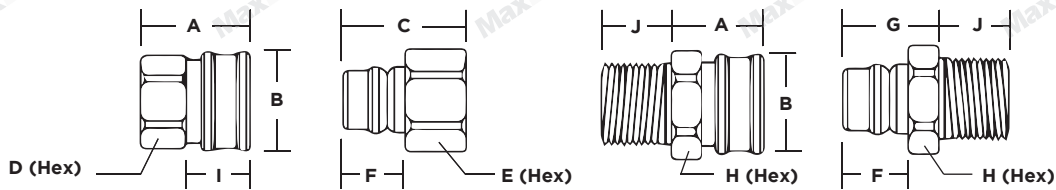
QRC 5 SERIES WITHOUT VALVE
