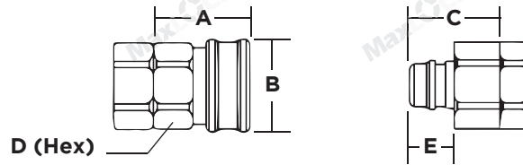
QRC 5 SERIES WITH VALVE (without end fitting)
